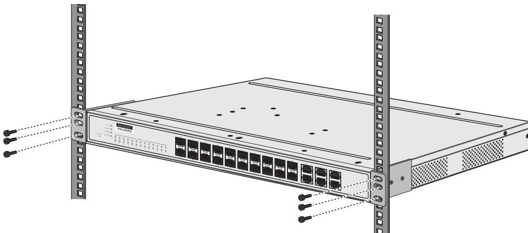
Figure 2.2 Installing the Switch
