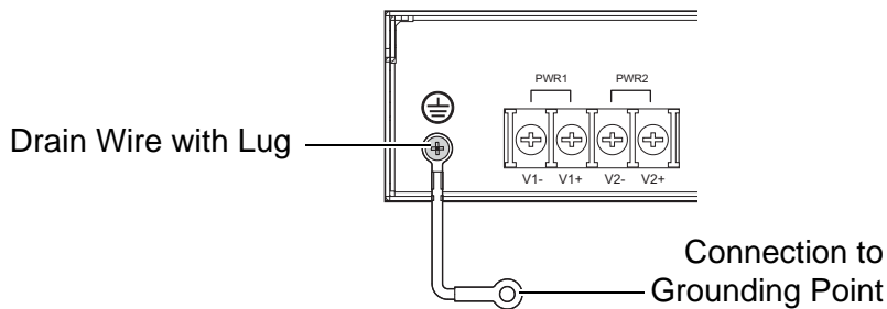
Figure 2.13 Grounding Connection
