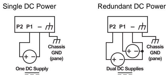
Figure 2.12 Power Wiring for EKI-9226G Series
