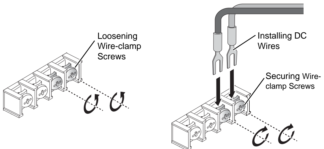
Figure 2.16 Installing DC Wires in a Terminal Block
